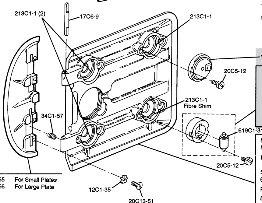
Figure 33. Standard and Baseplate Assembly (Exploded View)
