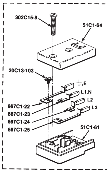
TERMINAL BLOCK
