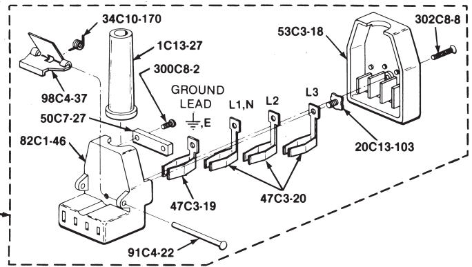
ATTACHMENT PLUG PATENT PENDING 523C1-100 SHOWN
